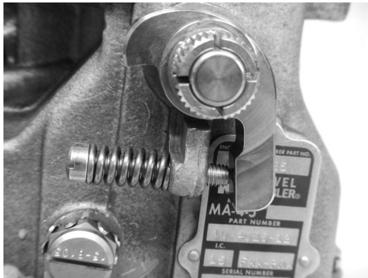
Figure 5-10a: Idle Position
