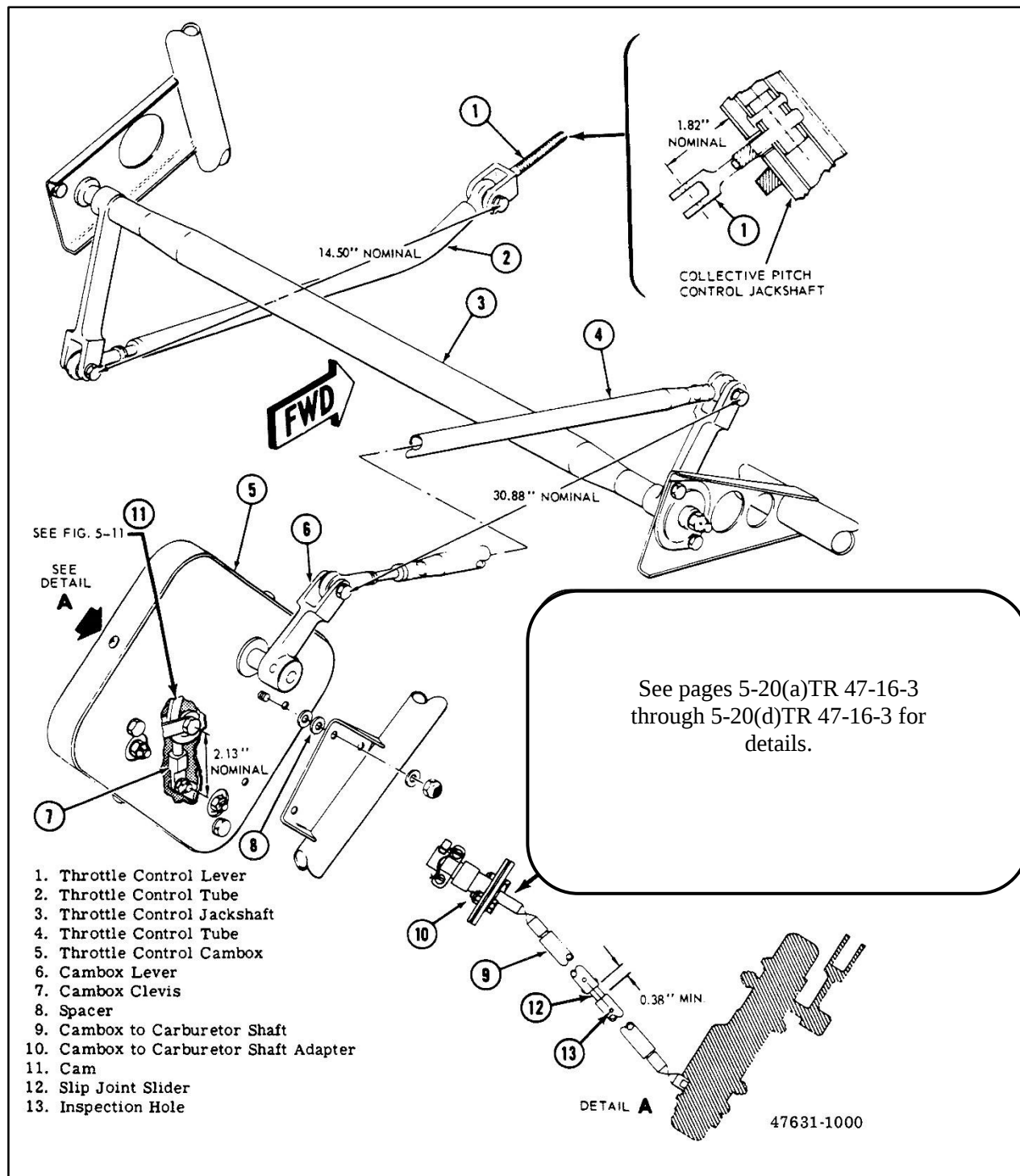
Figure 5-10. Throttle Control Installation (Sheet 1 of 2)
